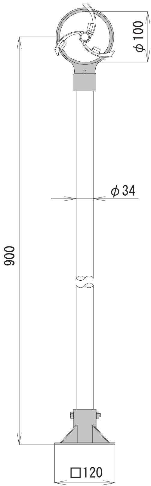
ATD34-100S(BP) (片面) ATD34-100W(BP) (両面)
